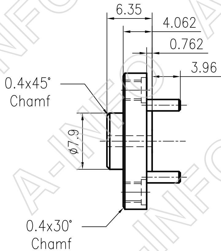
FUGP740 (equivalent to UG-387/U)
