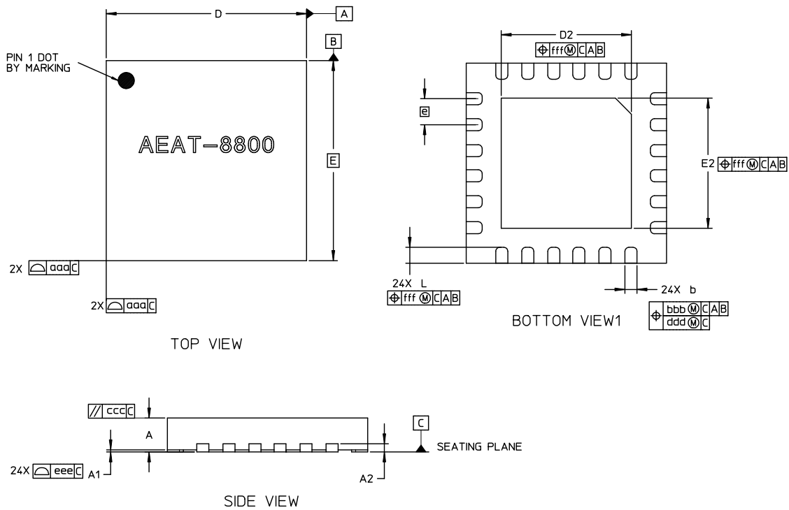
Figure 16 AEAT-8800, 24 QFN Dimensions
