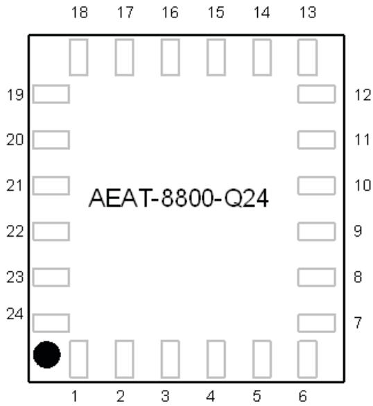
Figure 4 Pin Configuration for AEAT-8800-Q24
