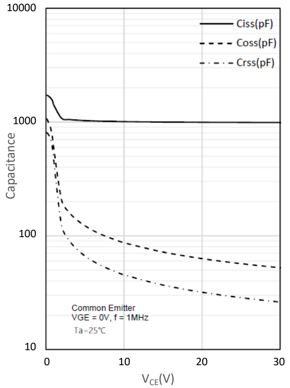
Fig. 10 Capacitance characteristics
