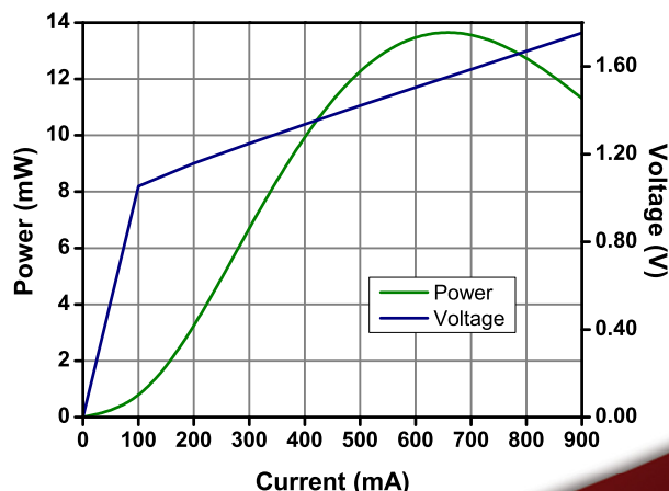
SLD1021S: Optical Power and Forward Voltage
