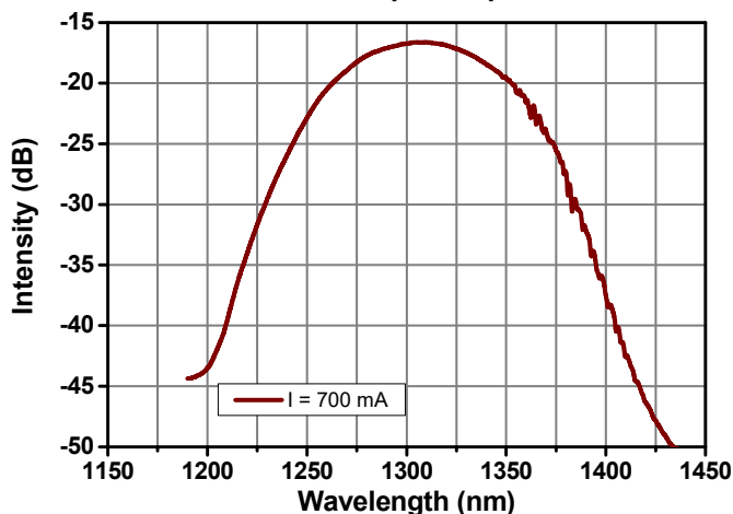
SLD1021S: Optical Spectrum
