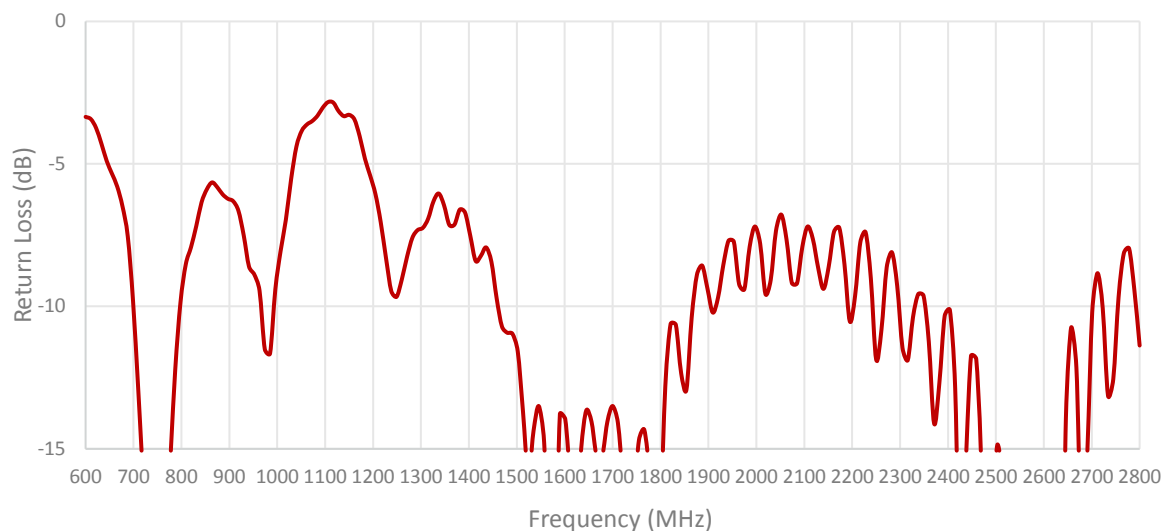
Cable 1: CELLULAR/LTE
