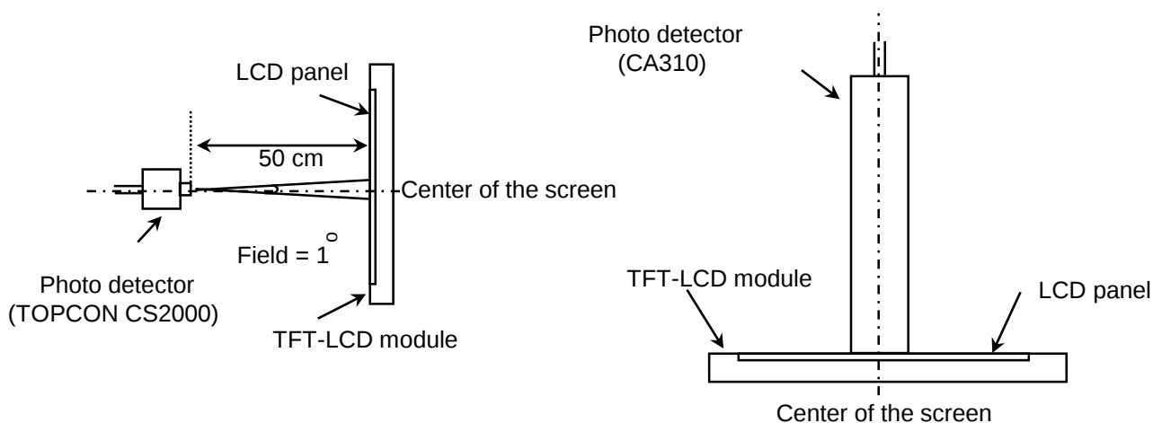
Figure 9. Measurement Set Up
