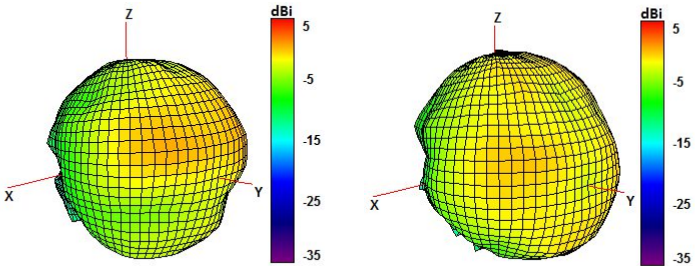
1950 and 2100 MHz Radiation pattern
