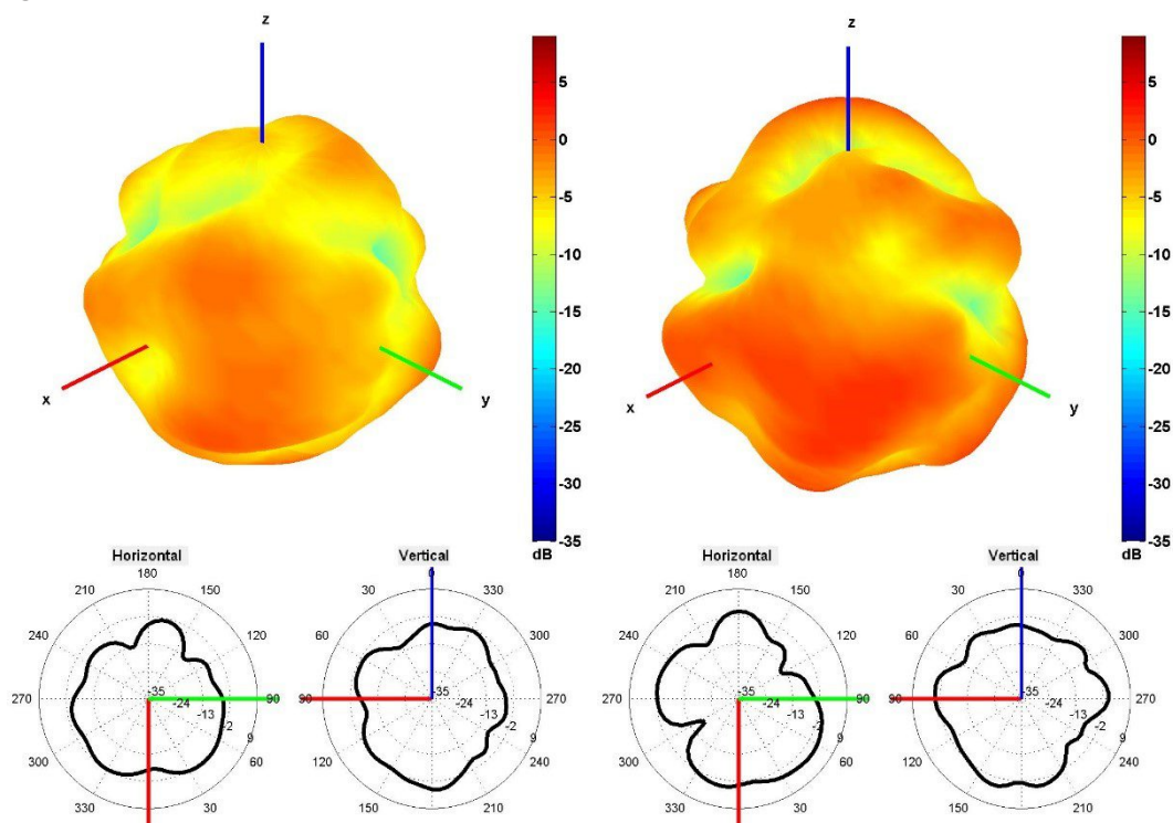
Cable 2: CELLULAR/LTE
