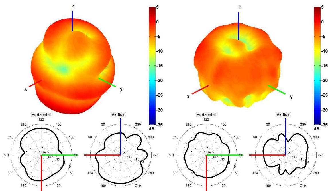
740 and 2500 MHz Radiation pattern
