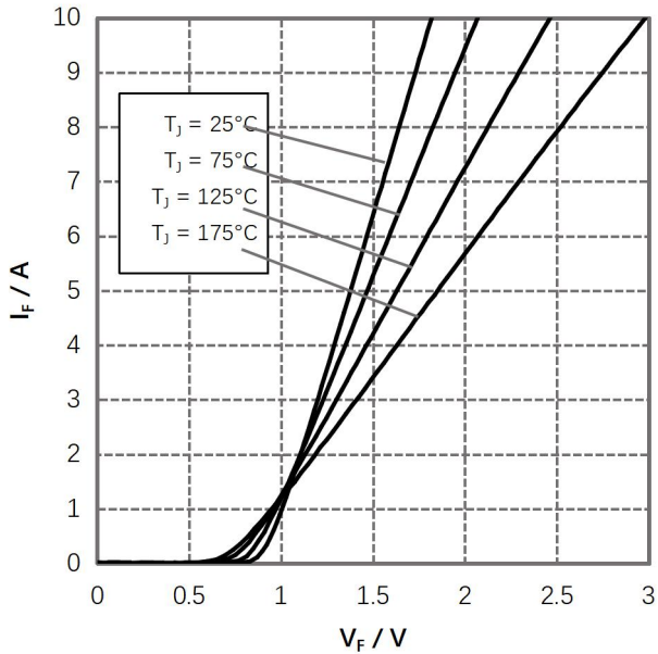
Figure 1. Forward Characteristics
