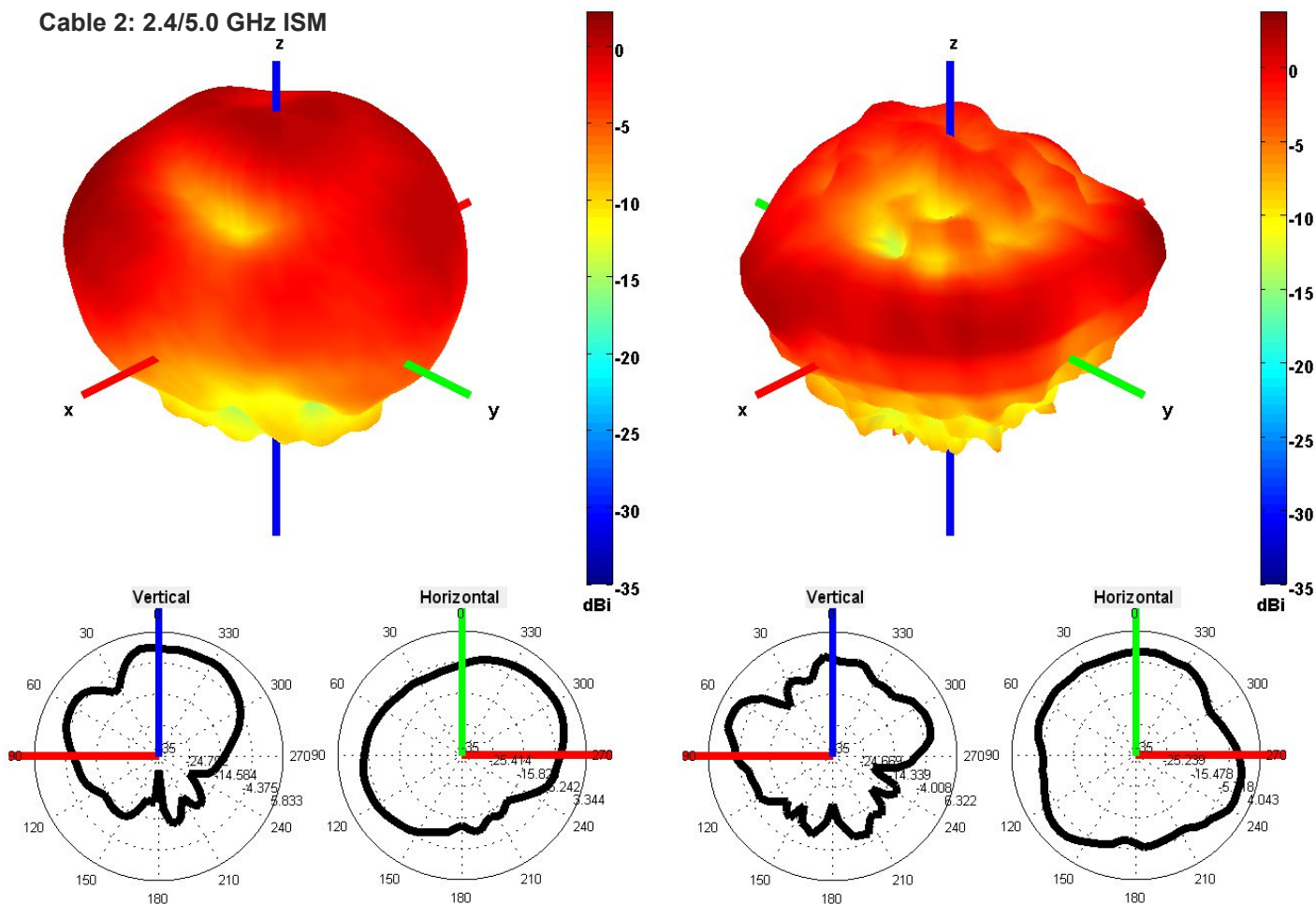
2450 and 5500 MHz Radiation pattern
