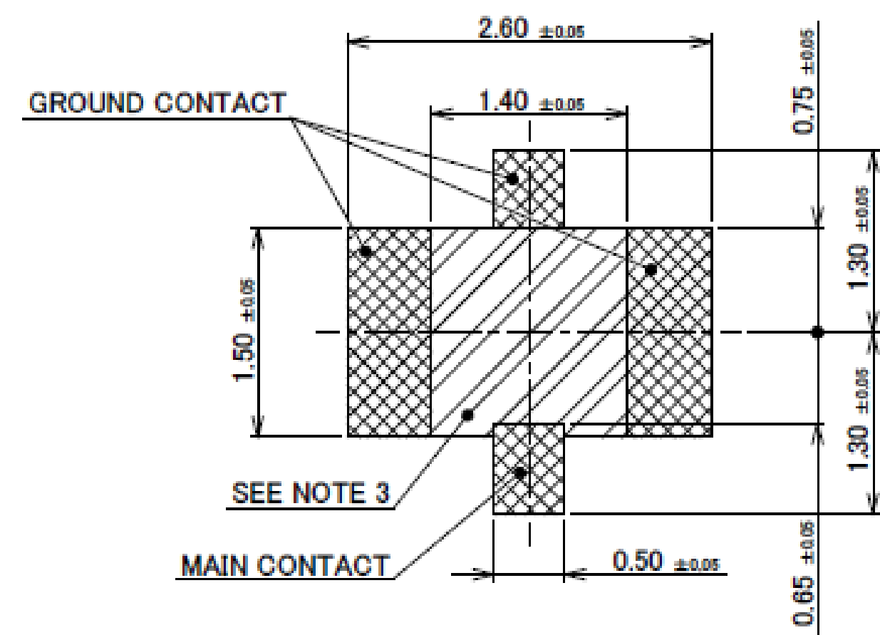
RECOMMENDED FOOTPRINT PATTERN
