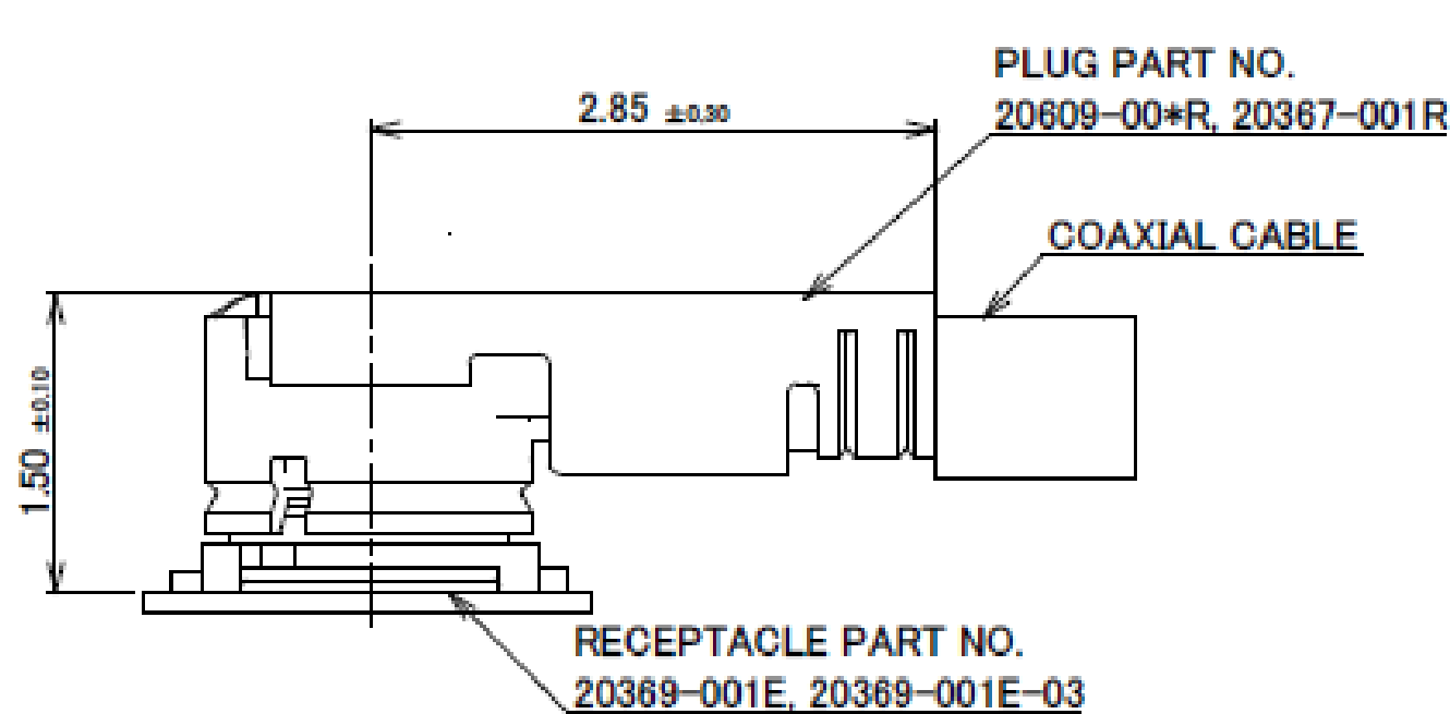
MATING CONDITION
