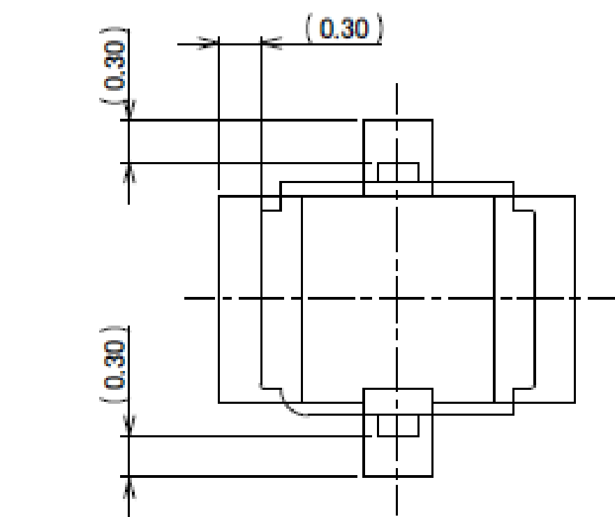
CONNECTOR ON RECOMMENDED FOOTPRINT PATTERN
