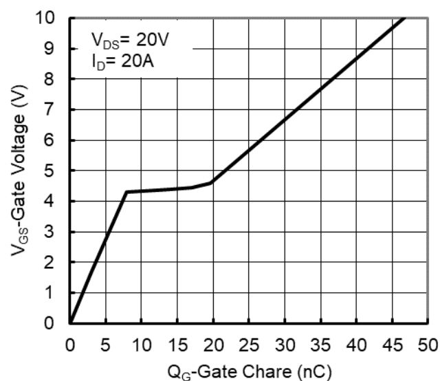
Figure 6. Gate Charge
