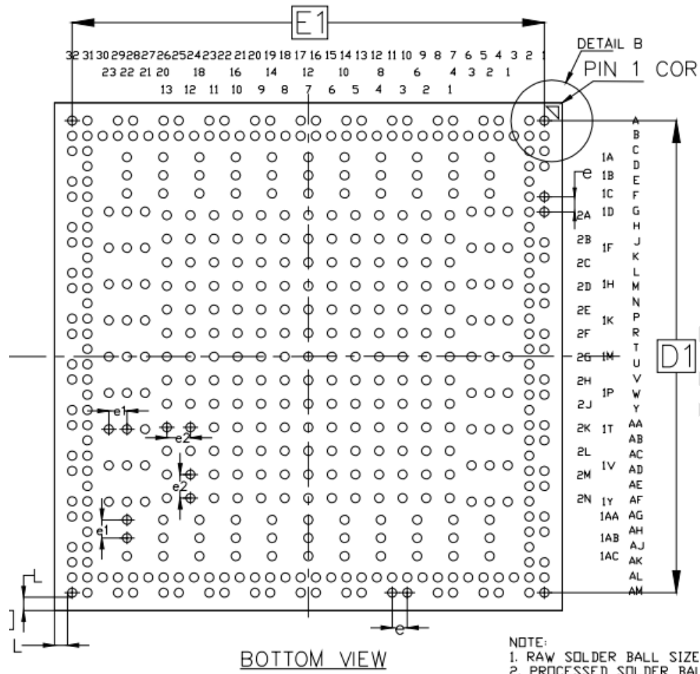
Fig. 2-2 RV1126B Package Bottom View
