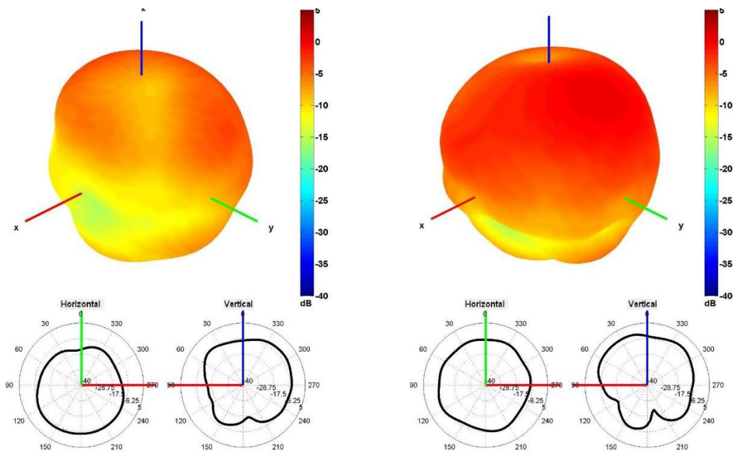
Cable 2: CELLULAR/LTE
