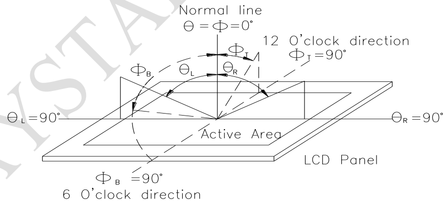
Fig. 12.1. Definition of viewing angle
