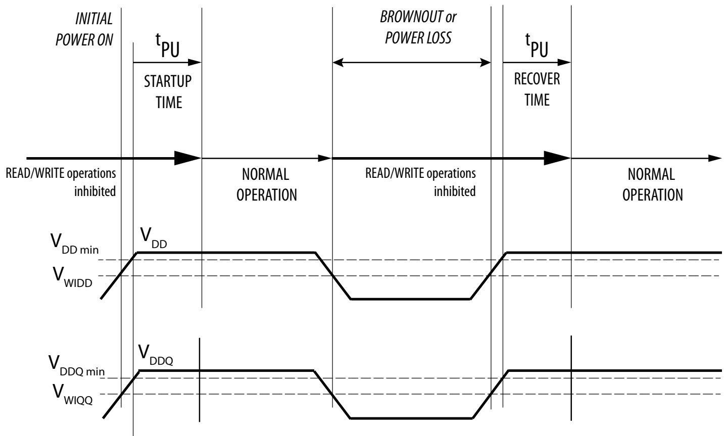
Figure 34 – Power-Up Timing
