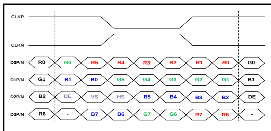
Figure 6.1.4 : 8-bit LVDS input ( IM[1:0]=01, LANSEL[1:0]=11, LVFMT=0(VESA) )
