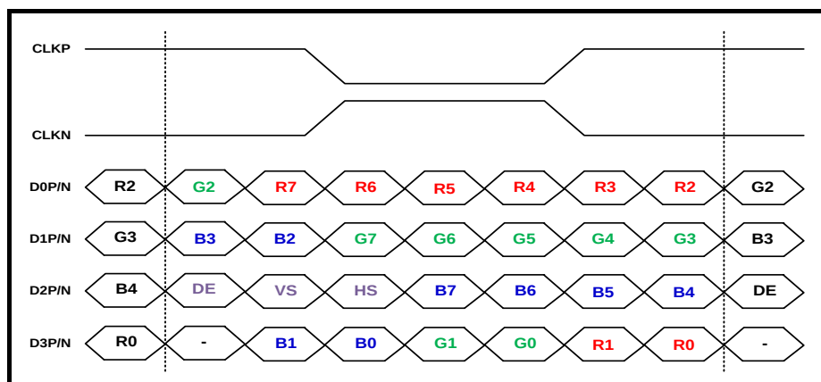
Figure 6.1.3 : 8-bit LVDS input ( IM[1:0]=01, LANSEL[1:0]=11, LVFMT=1(JEIDA) )
