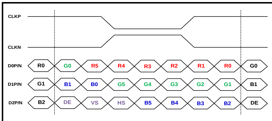
Figure 6.1.2 : 6-bit LVDS input ( IM[1:0]=01, LANSEL[1:0]=10, LVFMT=Don't care )
