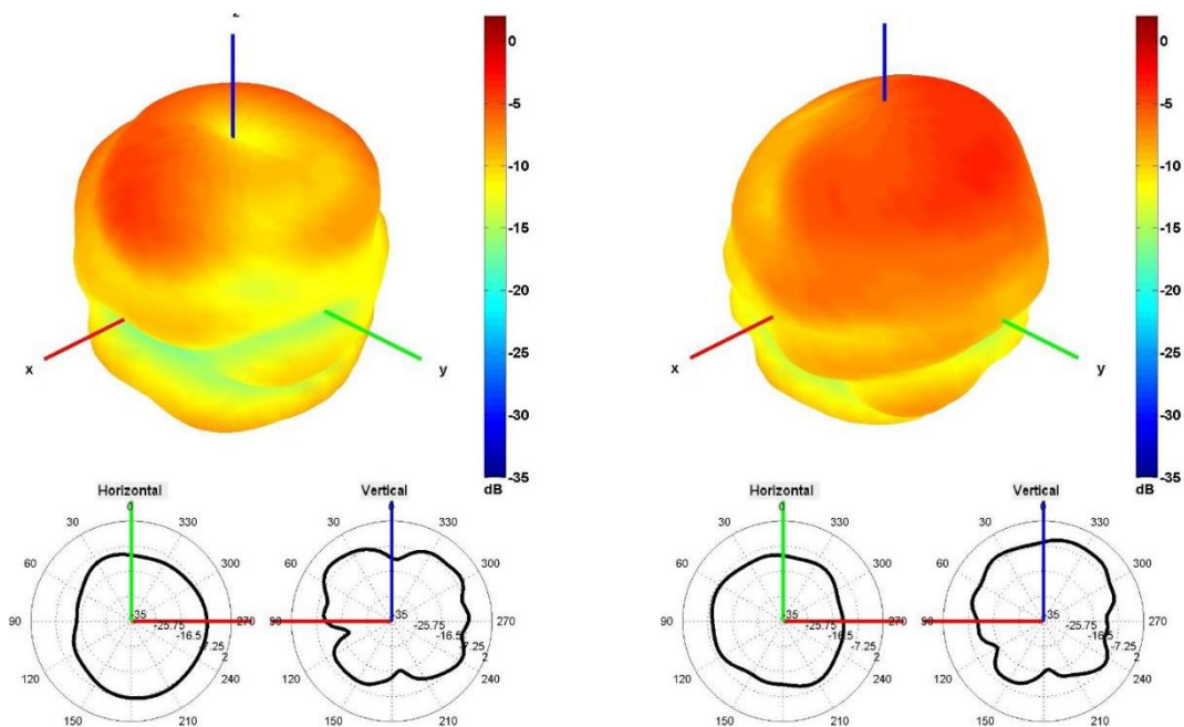
Cable 2: CELLULAR/LTE
