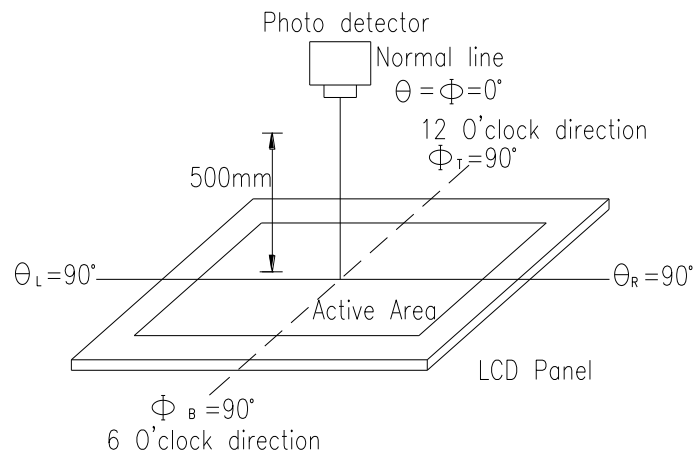
Fig. 11.2. Optical measurement system setup
