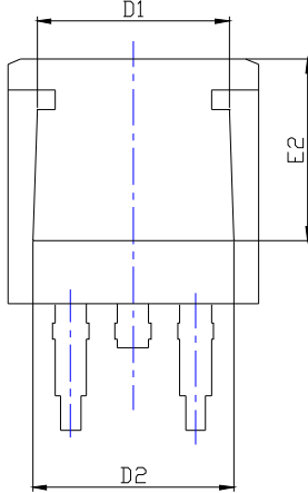
BOTTOM VIEW
