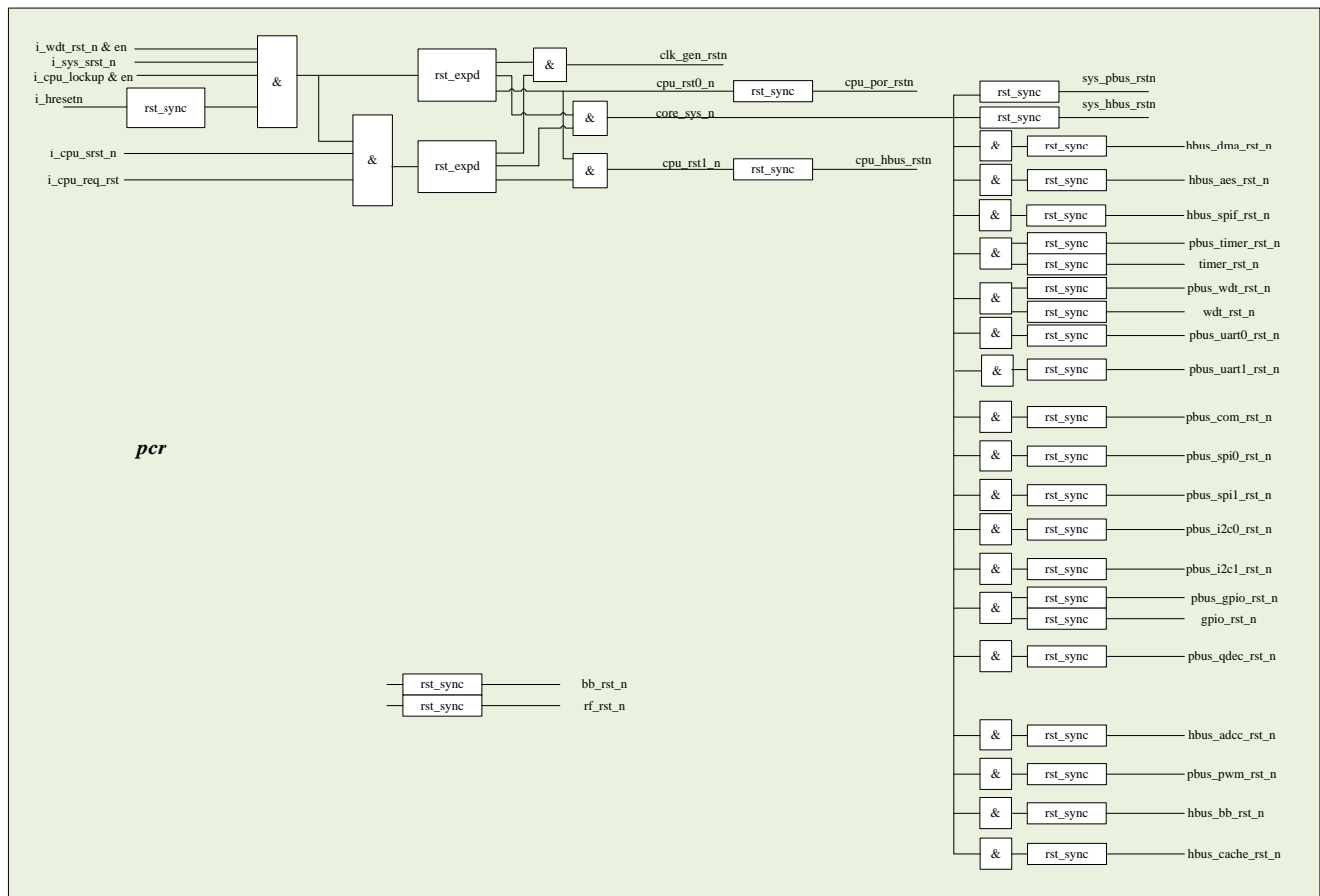
Figure 6: CMT4522 power, clock and reset
