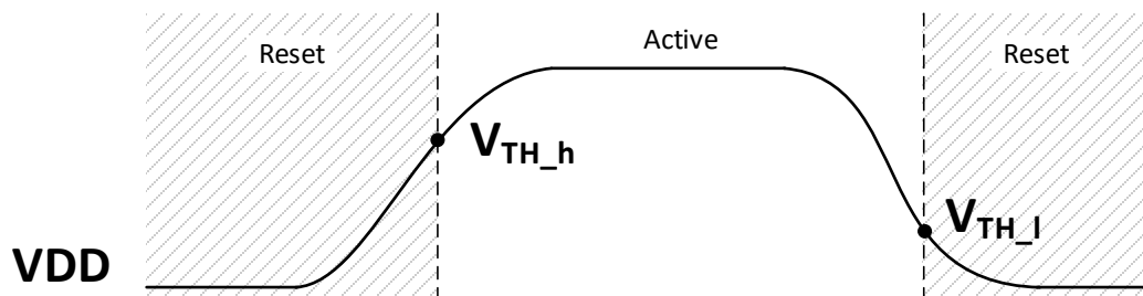
Figure 8: UVLO reset
