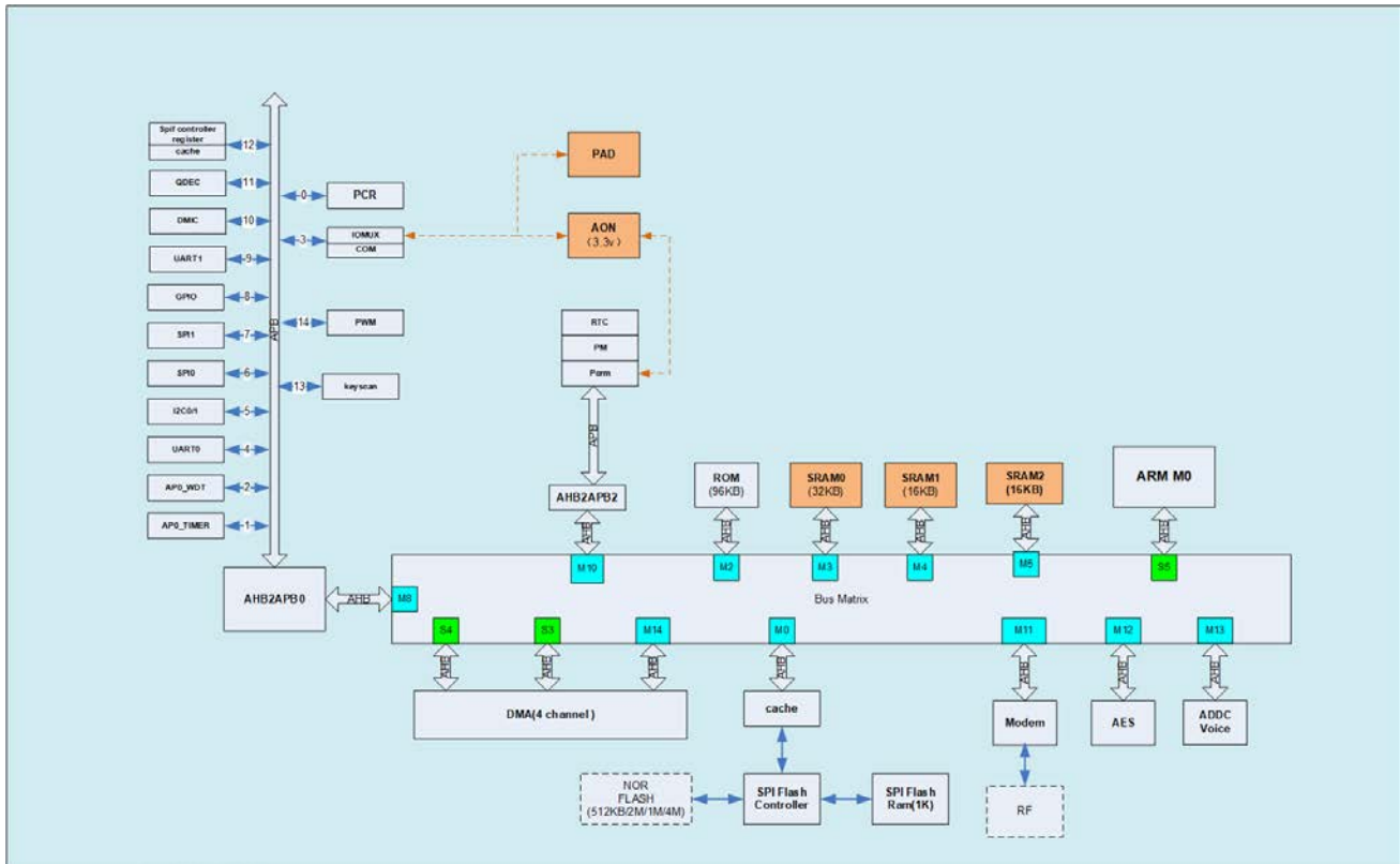
Figure 1: CMT4522 block diagram
