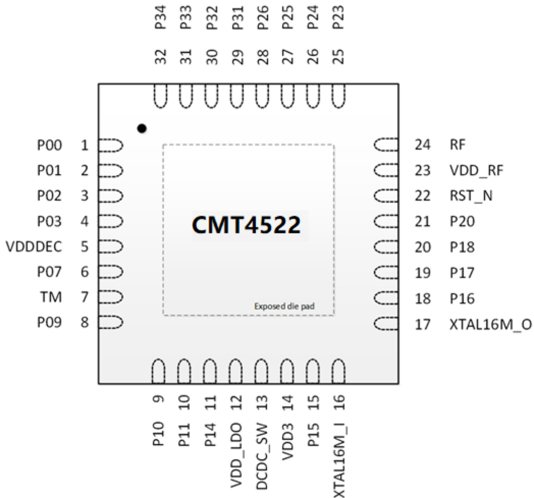
Figure 2: Pin assignment – CMT4522 QFN32 package
