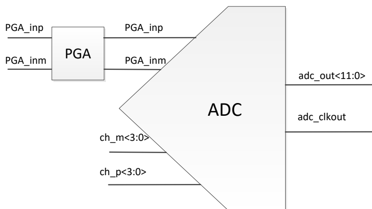
Figure 16: ADC
