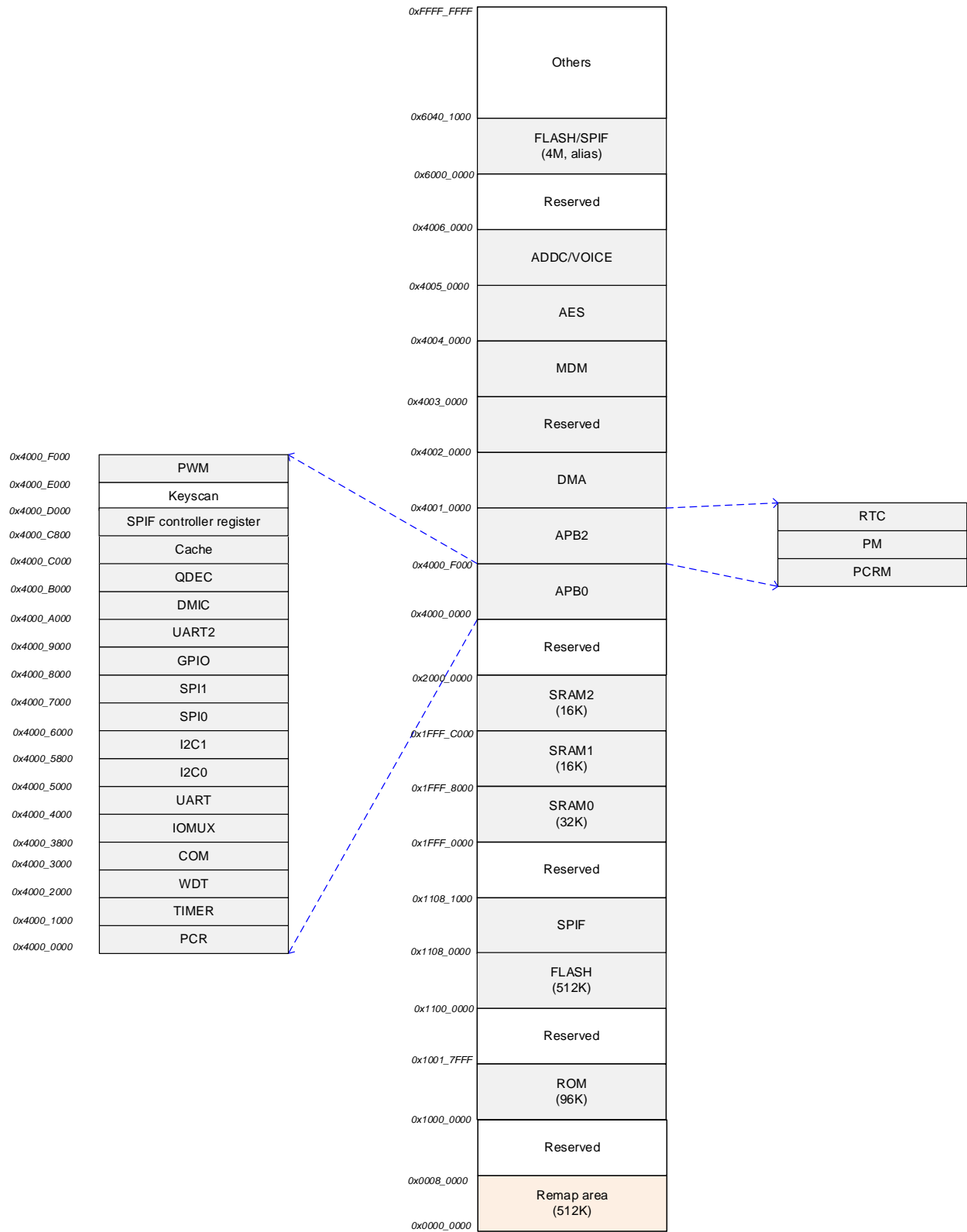
Figure 3: CMT4522 memory space
