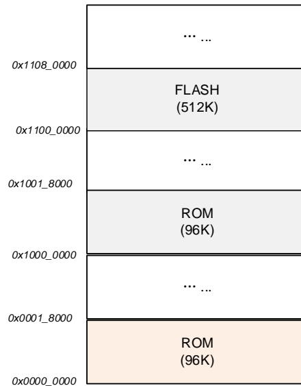
Figure 4: CMT4522 boot mode
