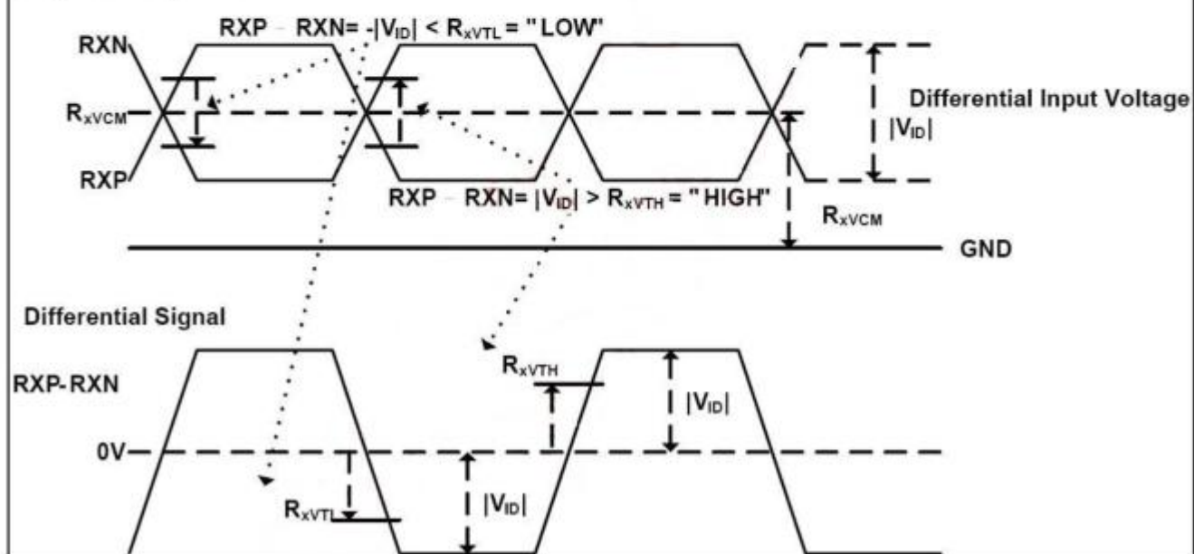
Single-end Signals
