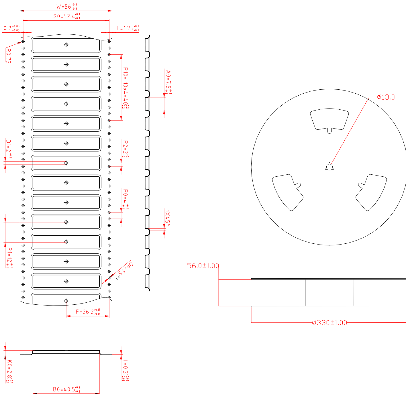
Tape and Reel Specifications
