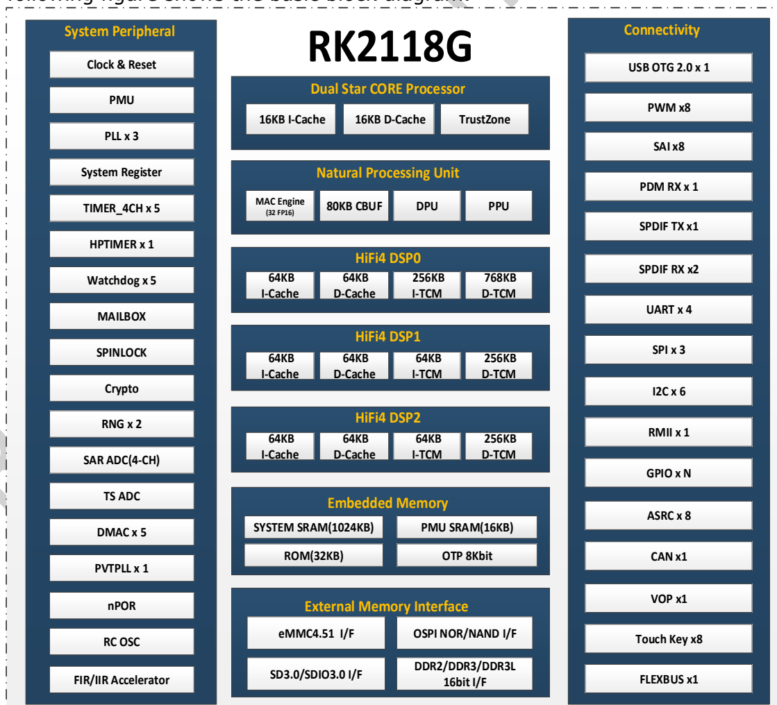
Fig.1-1 RK2118G Block Diagram
