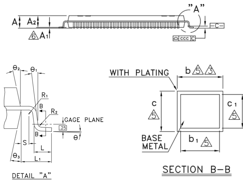
Fig.2-3 RK2118G Package Side View
