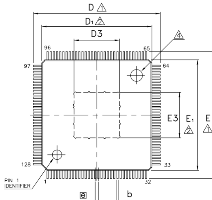
Fig.2-2 RK2118G Package Top View
