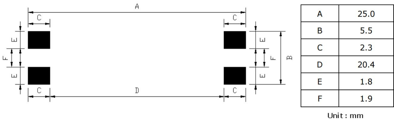
Solder Pads
