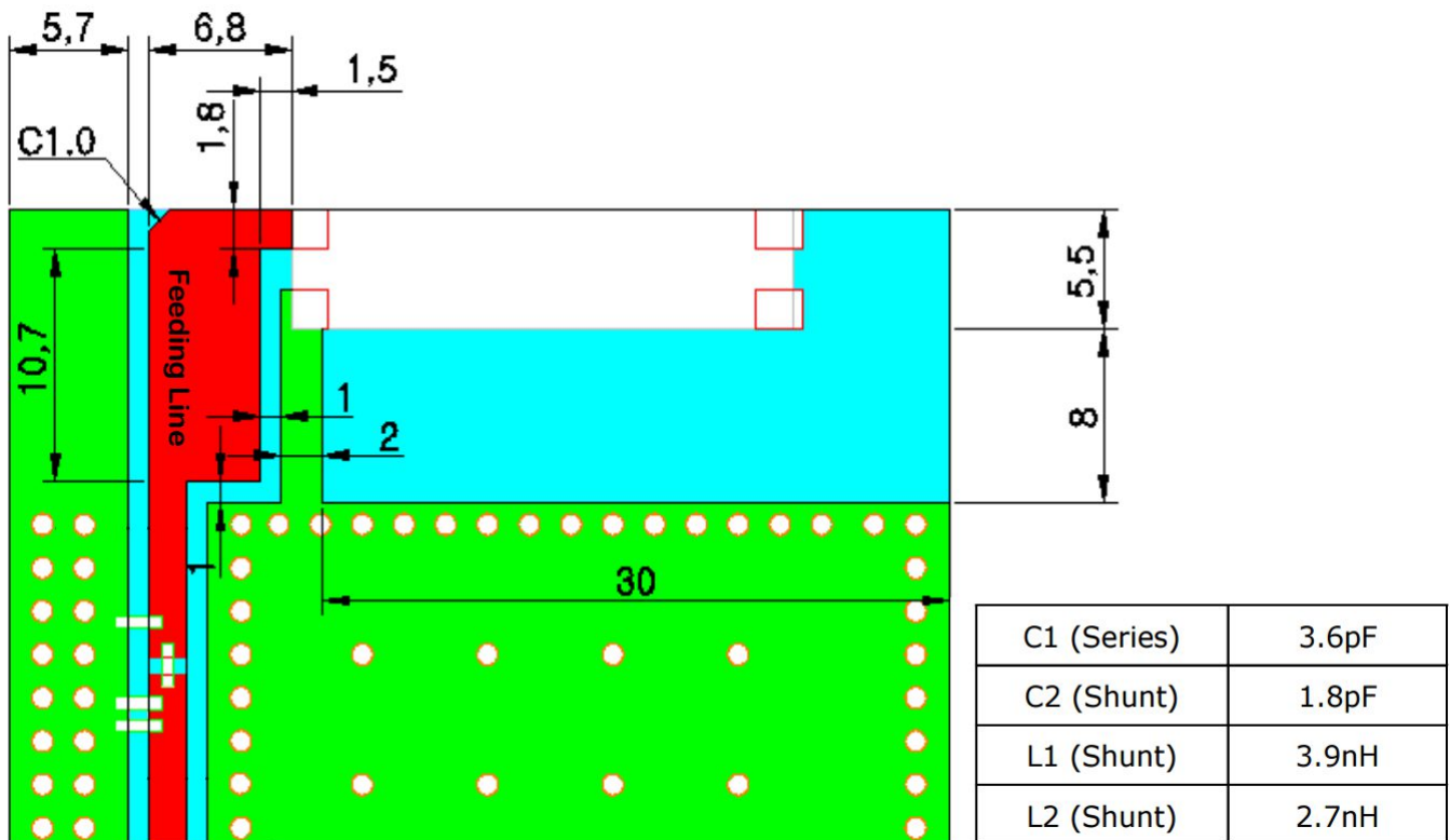
Layout and matching network
