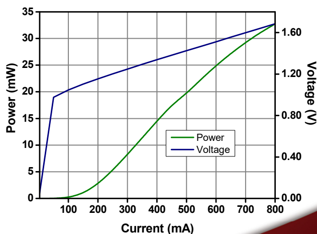
SLD1018S: Optical Power and Forward Voltage
