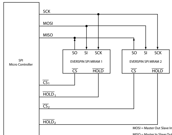
Figure 2 – System Configuration
