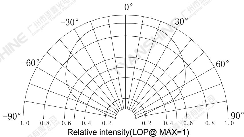
Beam Pattern
