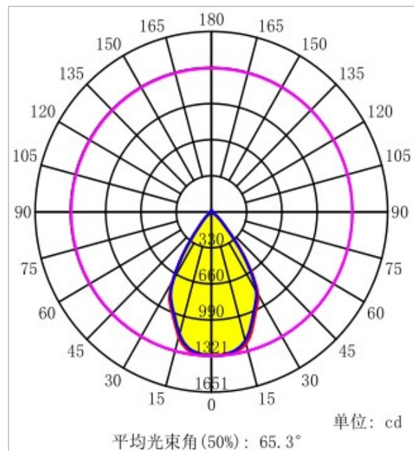
Part Number:KB-D4225-60RF-K
