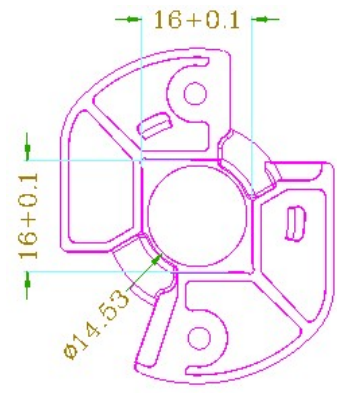
CREE-CXA1507/1515
