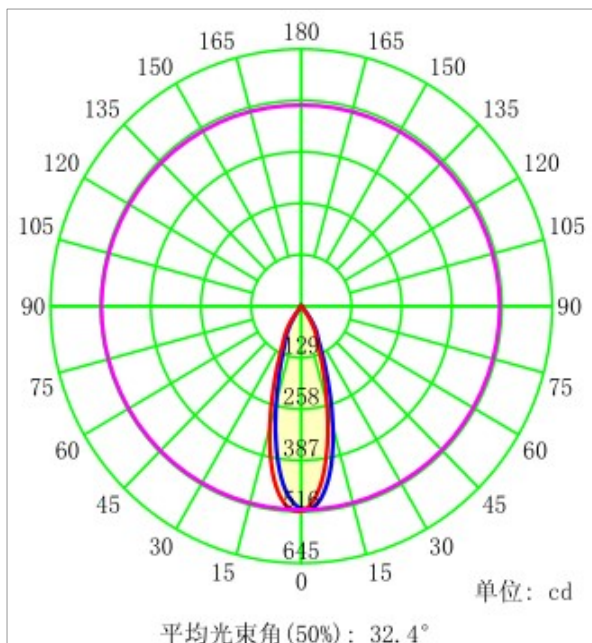
Part Number:KB-D4225-36RF-K
