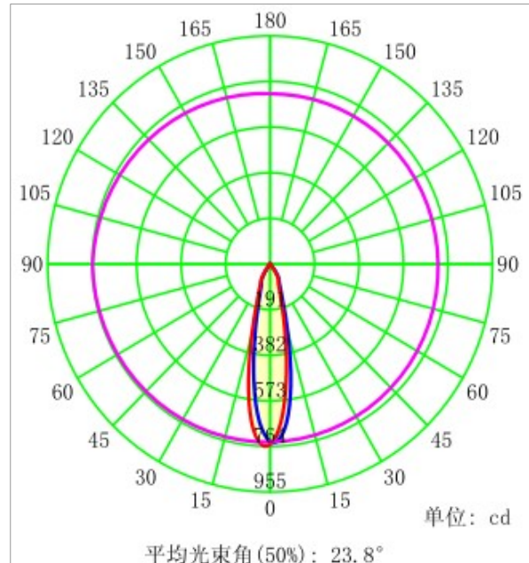
Part Number:KB-D4225-24RF-K
