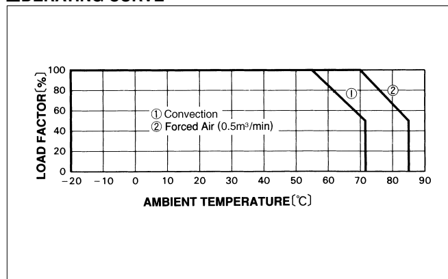
■ DERATING CURVE
