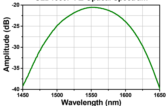
SLD1550P-A2 Optical Spectrum
