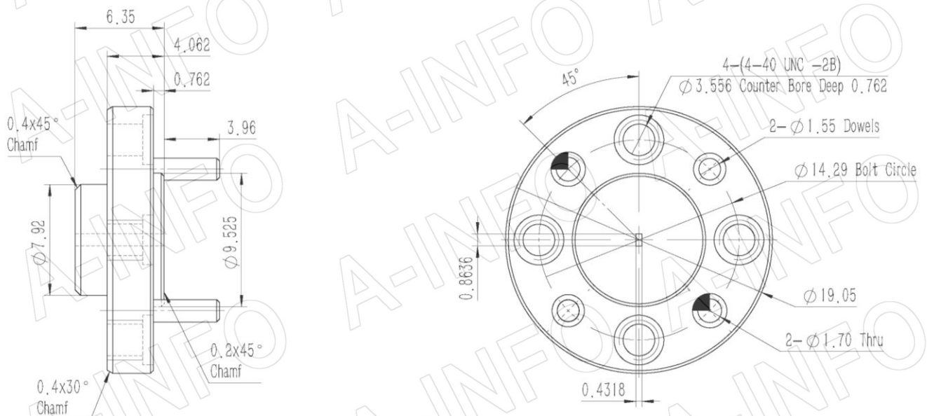
FUGP900 (equivalent to UG-387/U-M)
