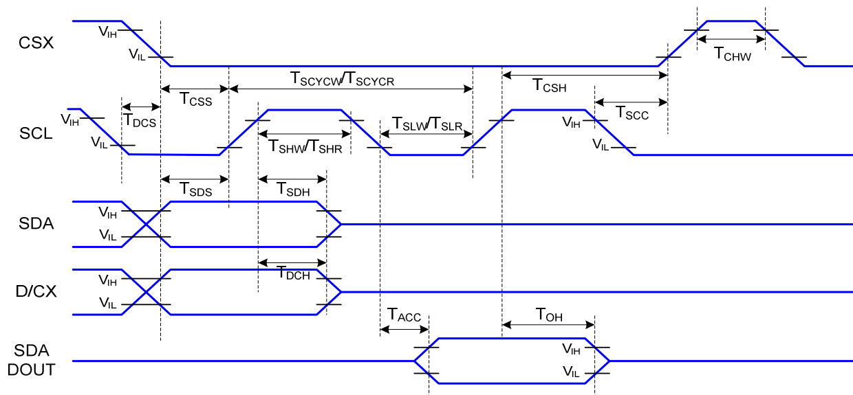
4-line Serial Interface Timing
