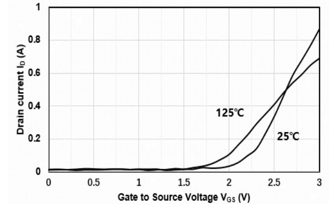
Figure2. Transfer Characteristics
