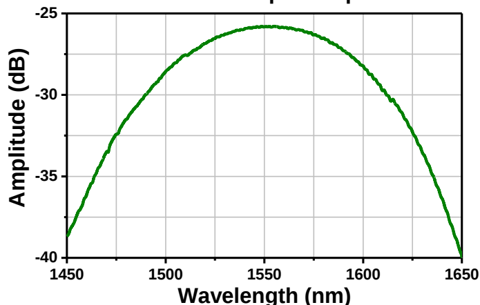
SLD1550P-A1: Optical Spectrum
