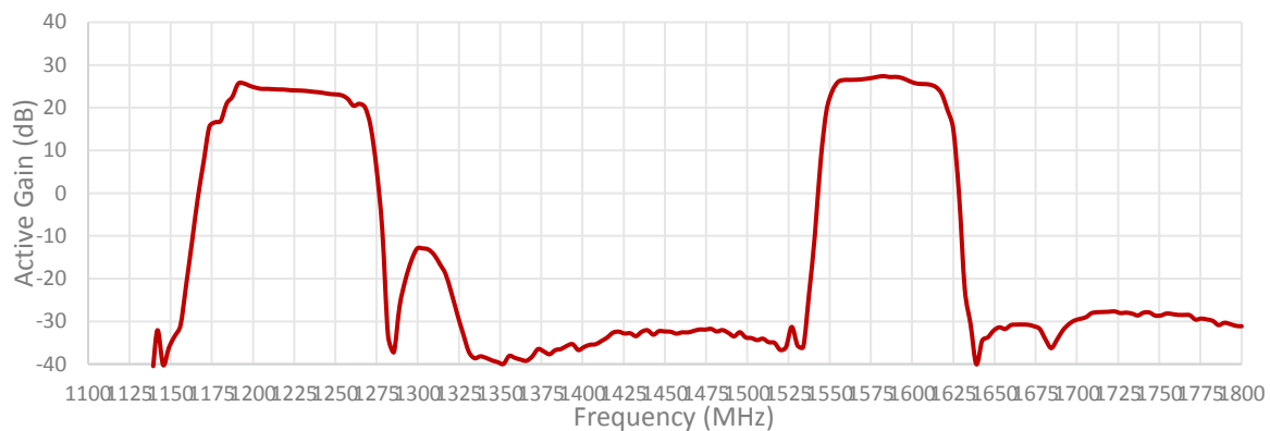
Cable 1: GNSS/L1L2
