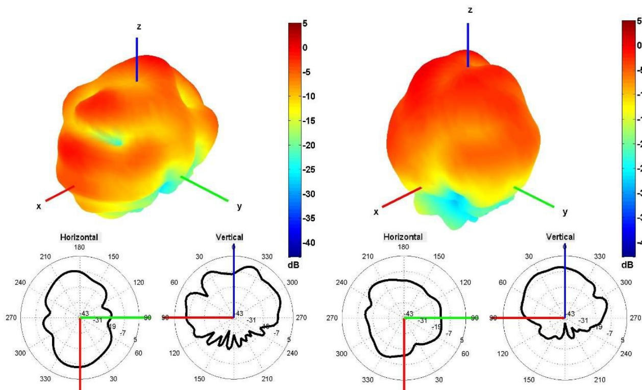
4500 and 5500 MHz Radiation pattern
