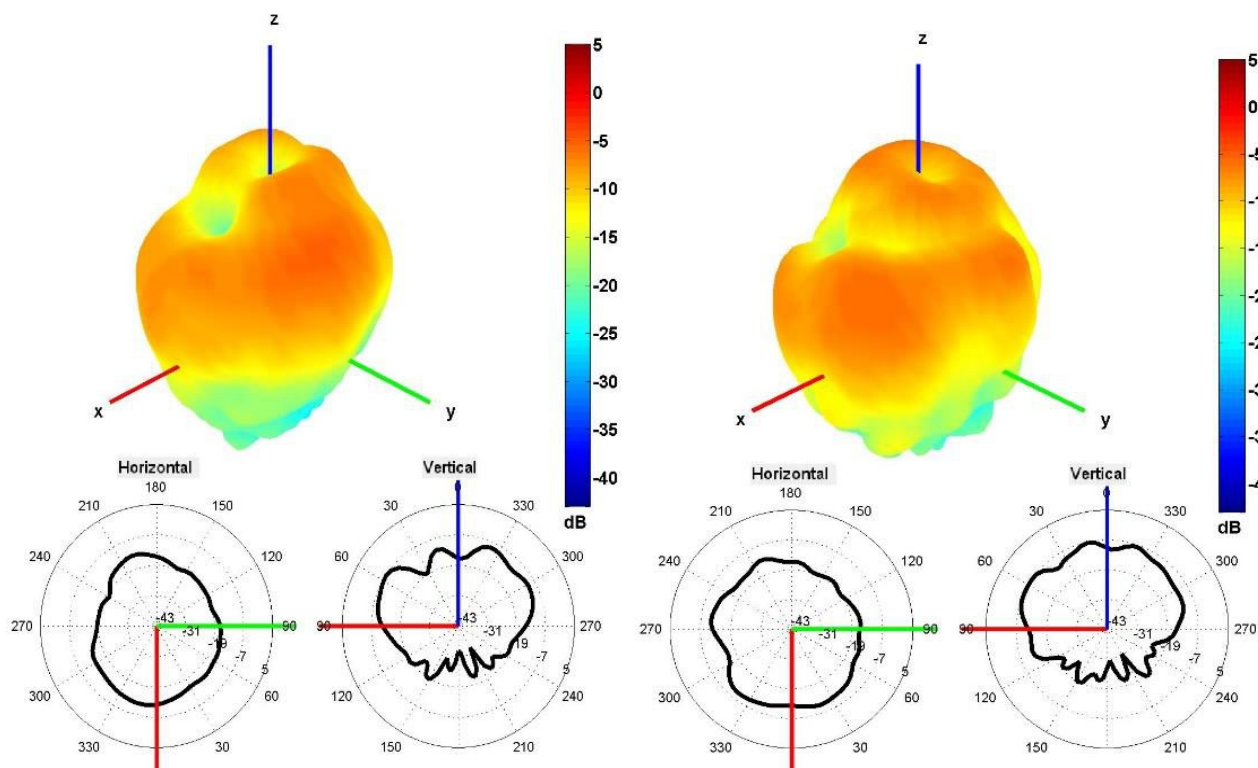
3350 and 3600 MHz Radiation pattern
