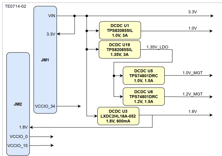
Figure 3: Power Distribution
