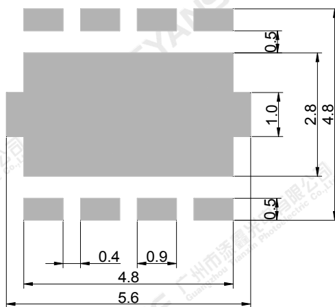
Recommended solder pad
