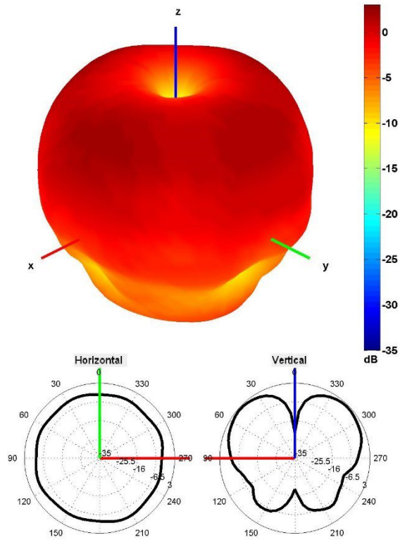
915 MHz Radiation pattern
