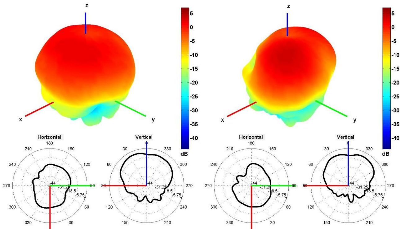
3350 and 3600 MHz Radiation pattern
