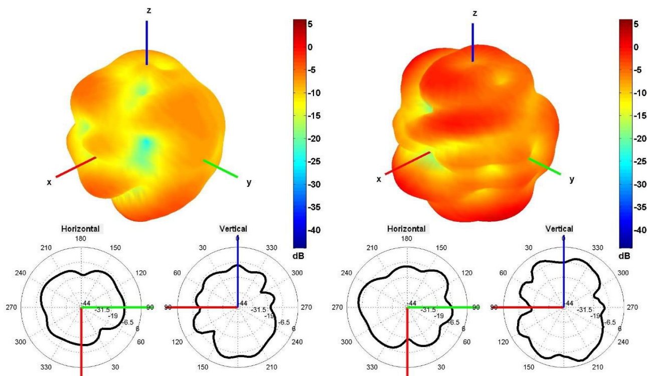
640 and 740 MHz Radiation pattern
