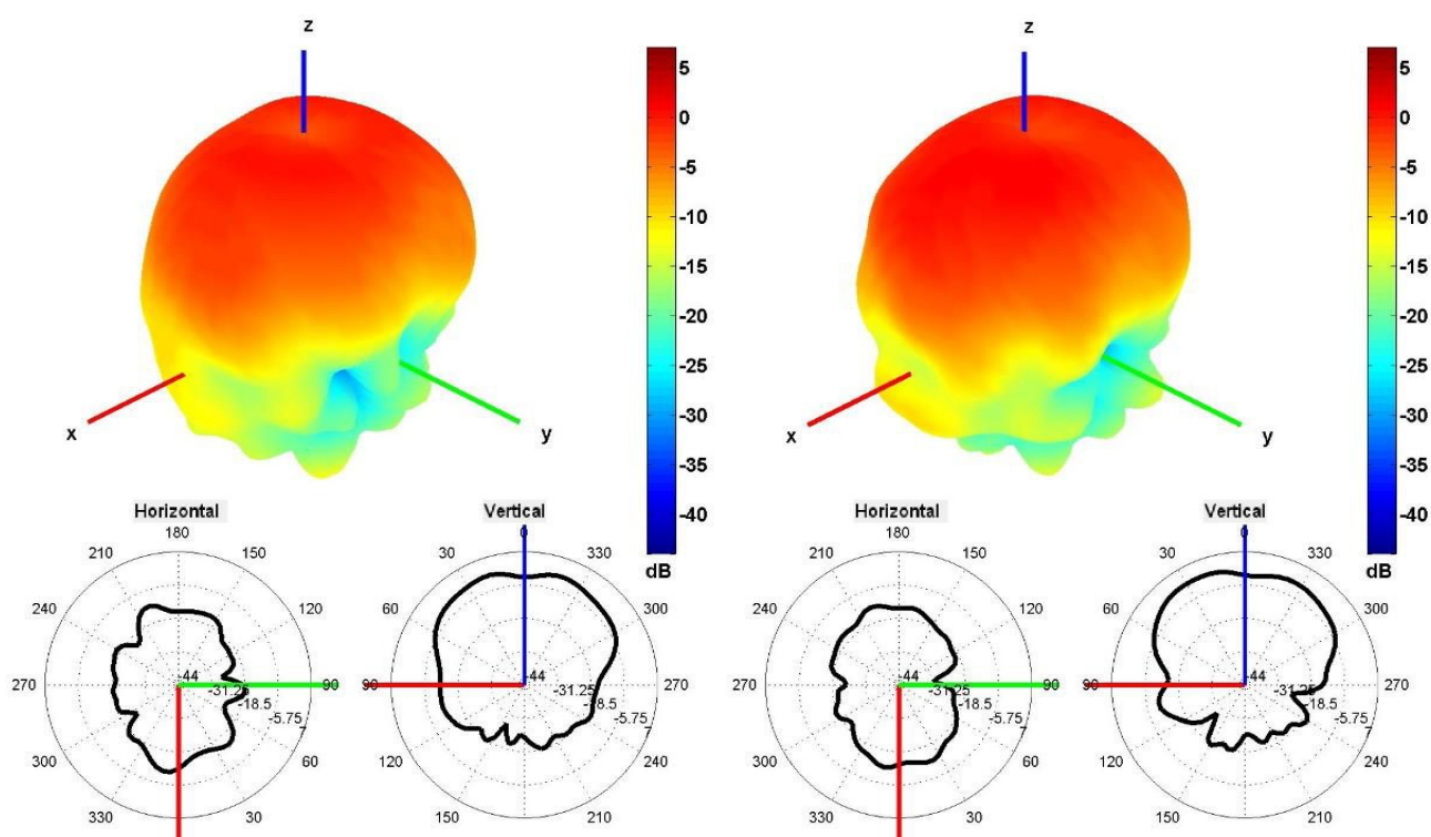
1950 and 2100 MHz Radiation pattern
