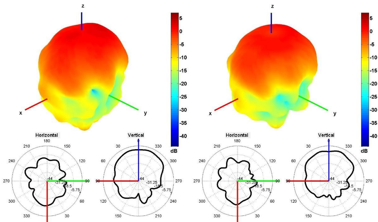
1750 and 1850 MHz Radiation pattern
