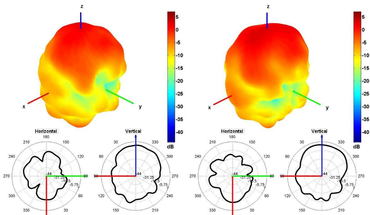
1500 and 1600 MHz Radiation pattern
