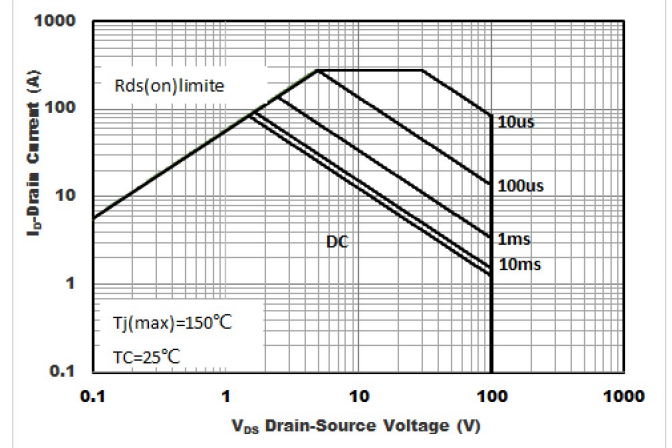
Figure8.Safe Operation Area
