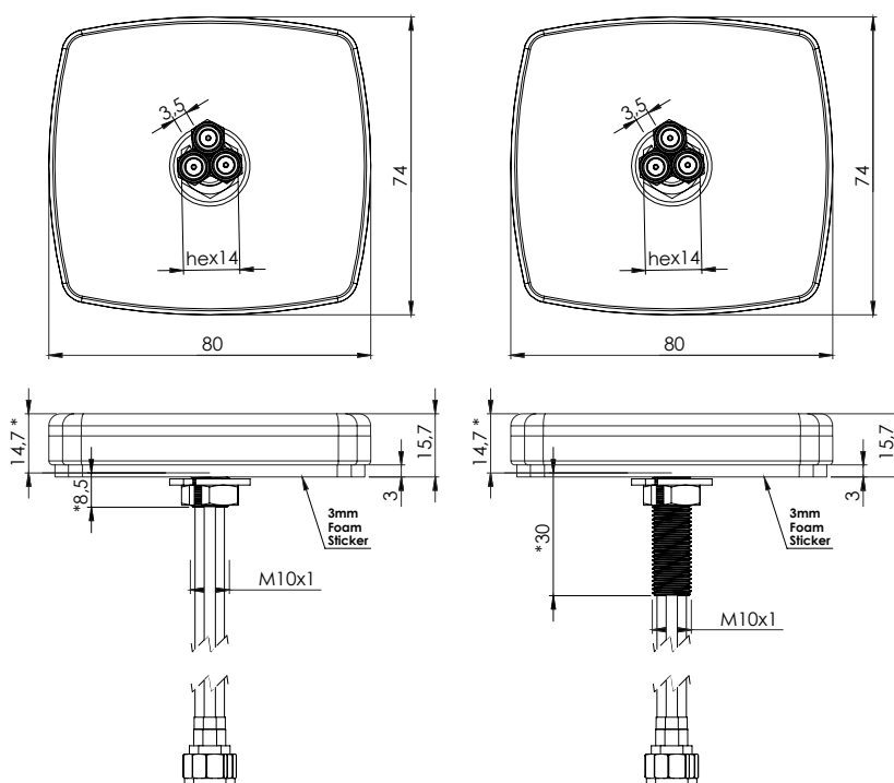
2J6041BGFa-TH8,5 8,5 mm Thread
