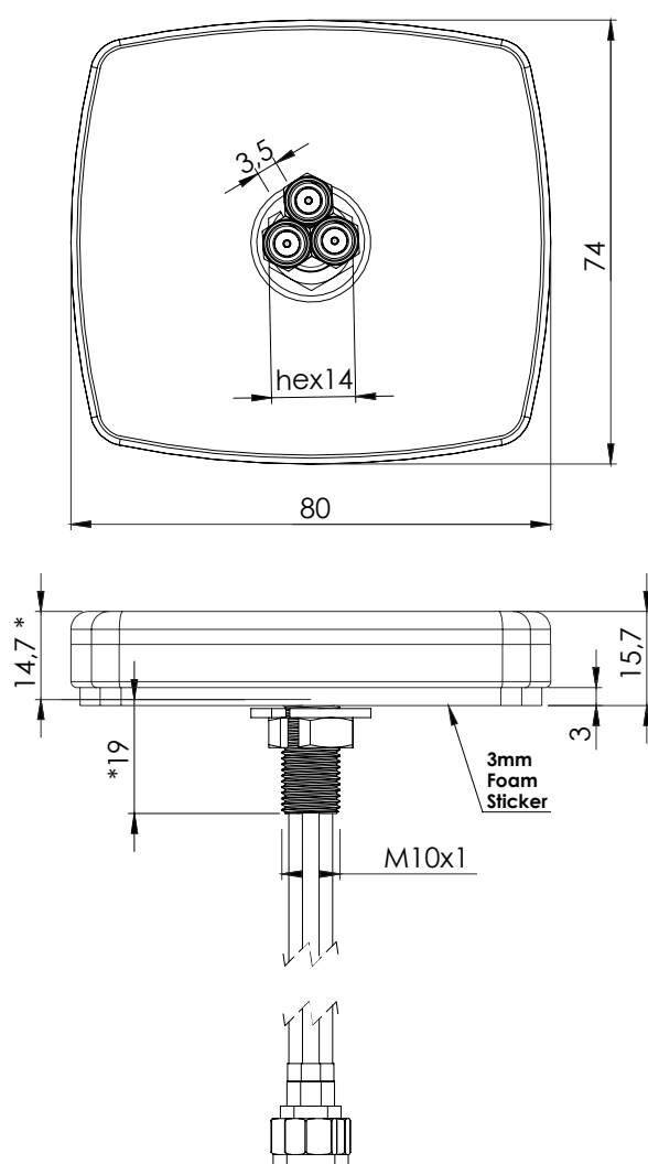
2J6041BGFa-TH19 19 mm Thread Default Option
