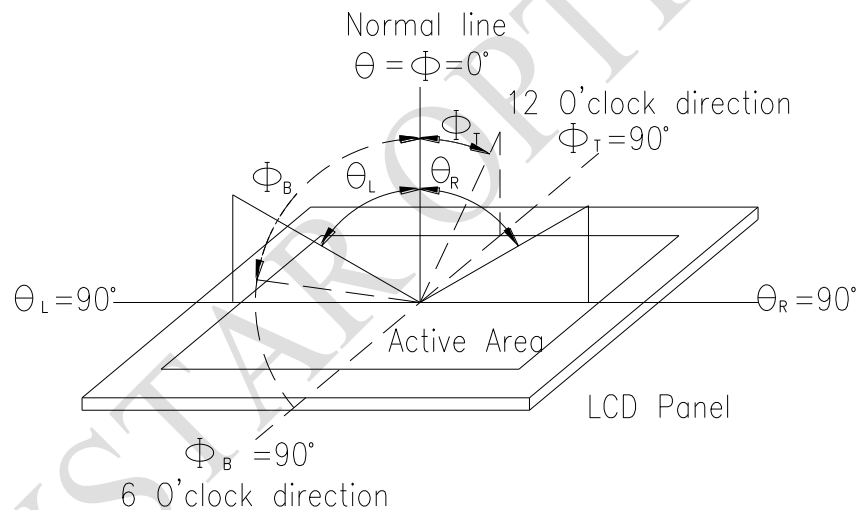
Fig. 9.1. Definition of viewing angle
