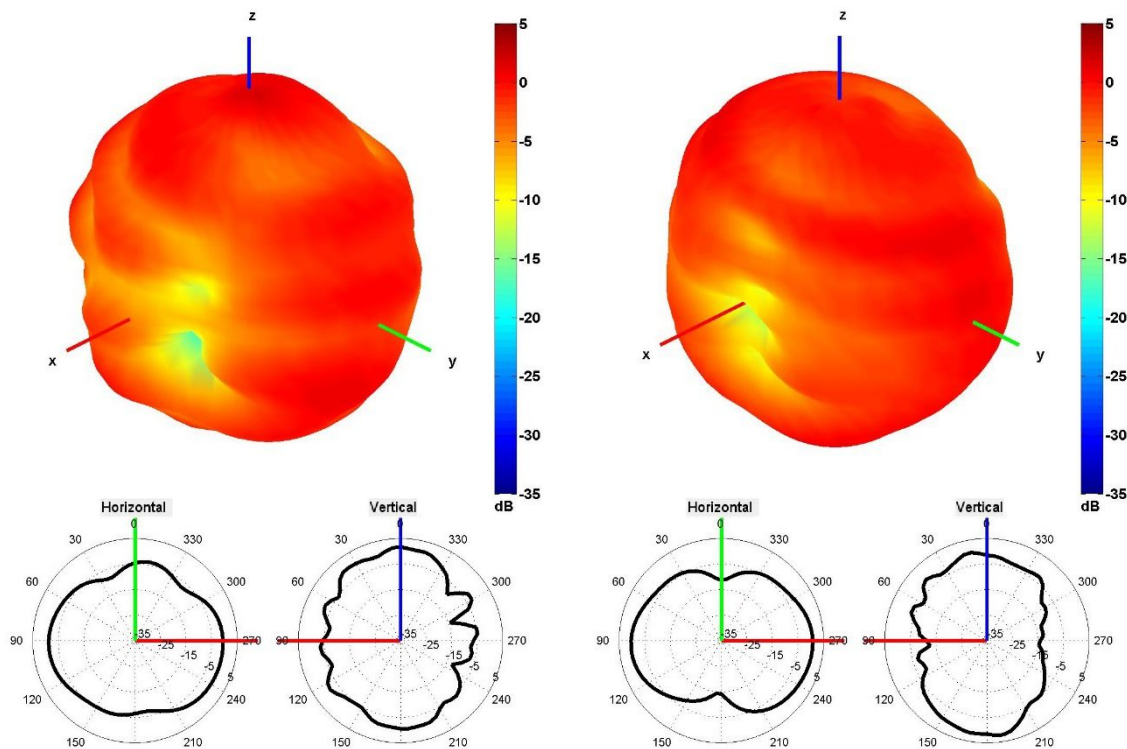
Cable 1: CELLULAR/LTE
