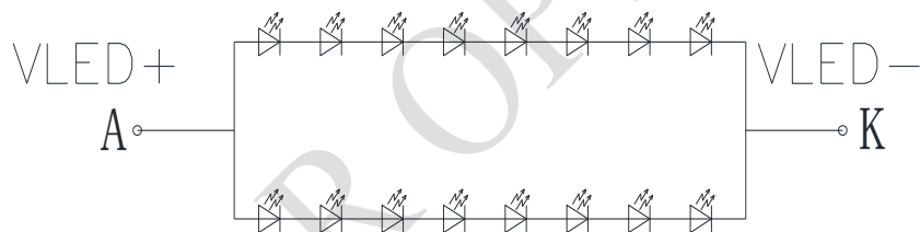
CIRCUIT DIAGRAM(8*2Dice)
