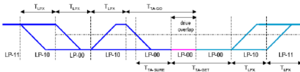
Figure 4.4 : Turnaround Procedure
