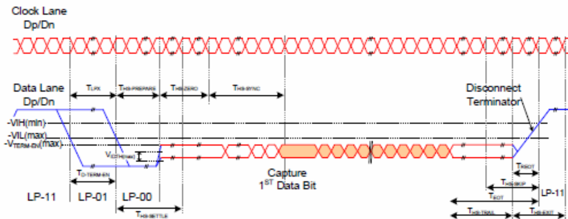
Figure 4.3 : Timing of high-speed data transmission in bursts
