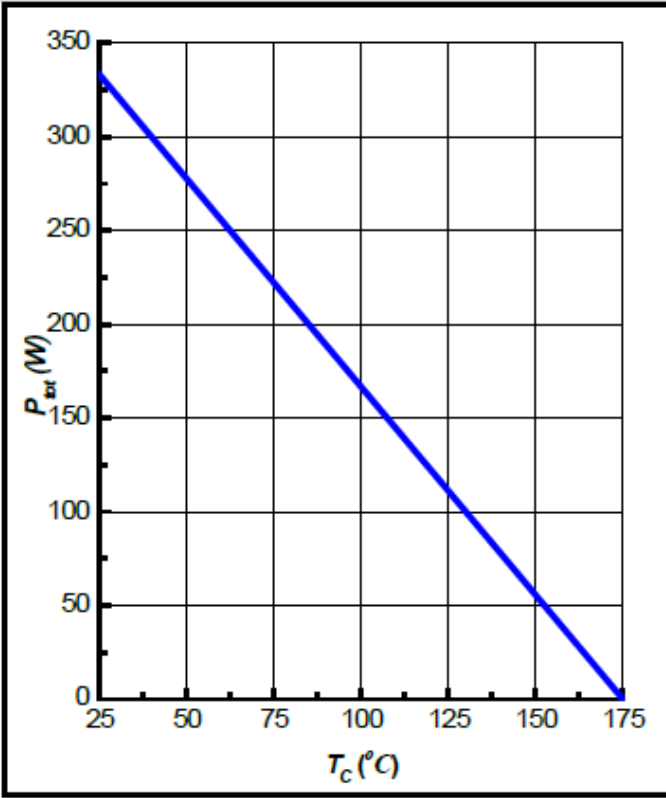
Figure 3. Power Derating
