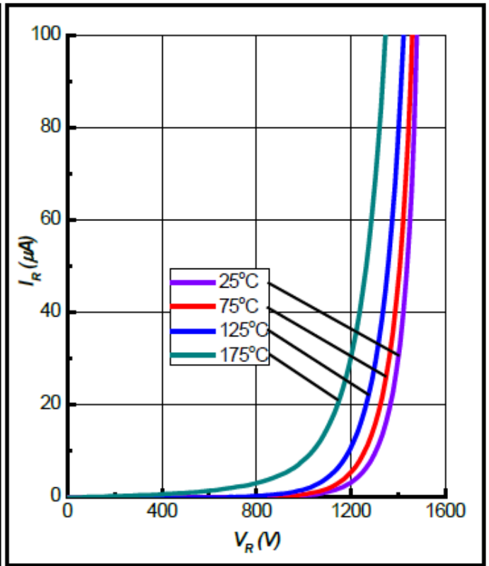
Figure 2. Reverse Characteristics
