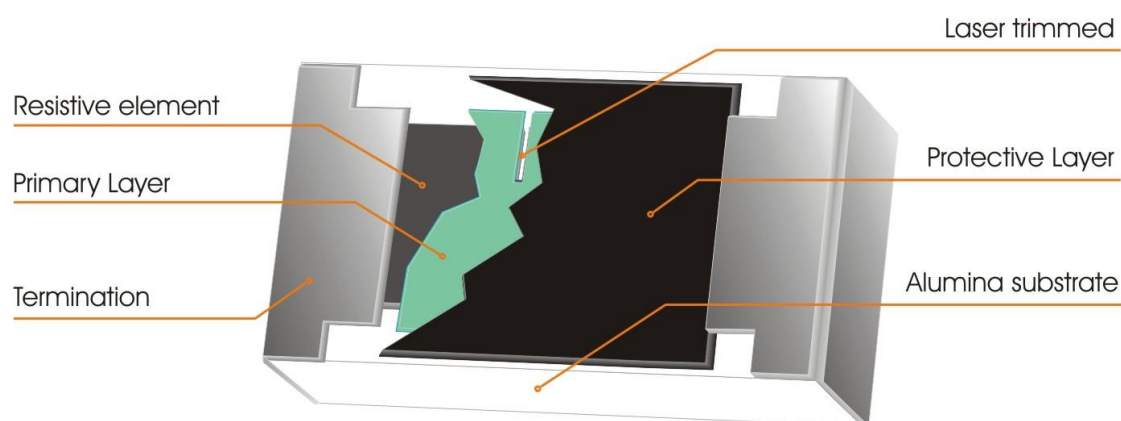
Fig 1. Construction of Chip-R WR01X
